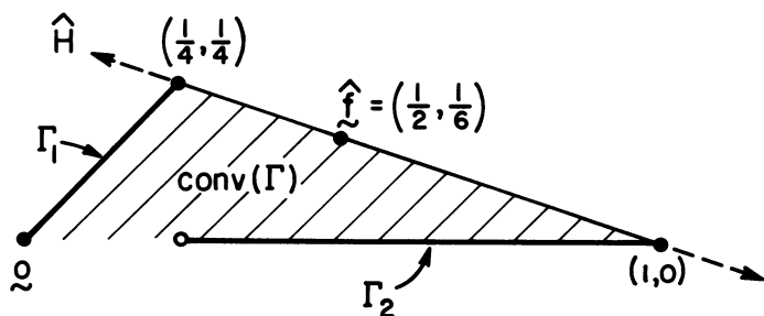
FIG. 2. In Example 2 with K = 2 the set \Gamma is the union of 0 = \{f_\theta: \theta \in (0, y_1)\} , \Gamma_1 = \{f_\theta: \theta \in [y_1, y_2]\} and \Gamma_2 = \{f_\theta: \theta \in [y_2, \infty)\} . Again \text{conv}(\Gamma) is a closed triangular region.
